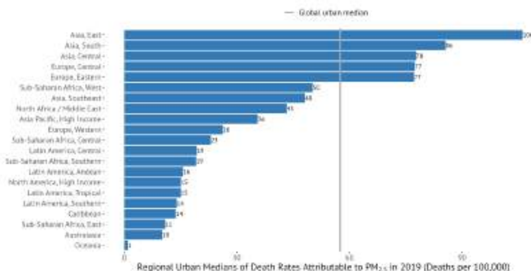
FIGURE 6 Regional urban medians of PM 2.5 attributable death rates in 2019.
